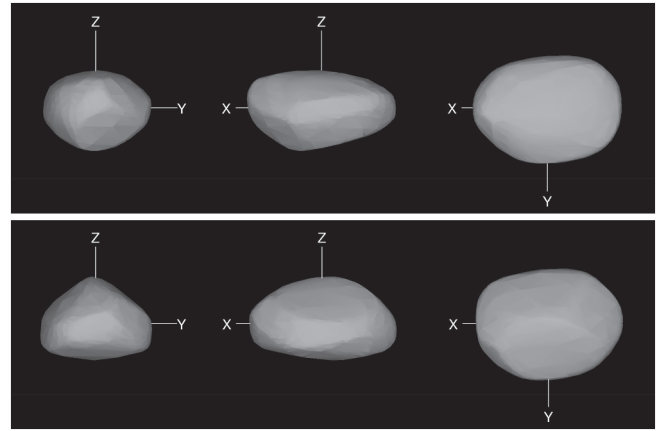
Fig. 26. Convex shape models of (56048) 1998 XV39 for the pole solutions (L_1, B_1) = (83^\circ, +31^\circ) (upper panel) and (267^\circ, +10^\circ) (lower panel).
