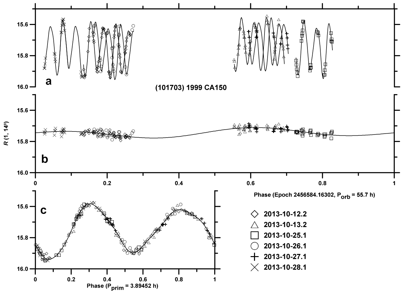
Fig. 28. Lightcurve data of (101703) 1999 CA150 from 2013. (a) The original data showing all the lightcurve components, folded with the orbital period. (b) The secondary rotational lightcurve component, derived after subtraction of the primary lightcurve component. Mutual events were not detected. (c) The primary lightcurve component.
