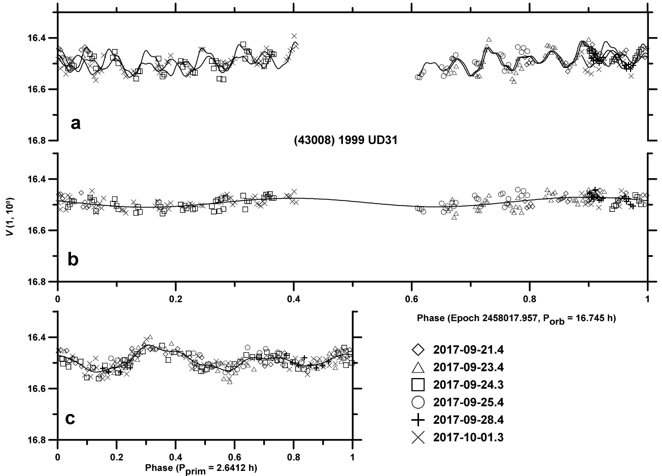
Fig. 15. Lightcurve data of (43008) 1999 UD31 from 2017. (a) The original data showing all the lightcurve components, folded with the orbital period. (b) The secondary rotational lightcurve component, derived after subtraction of the primary lightcurve component. Mutual events did not occur. (c) The primary lightcurve component.
