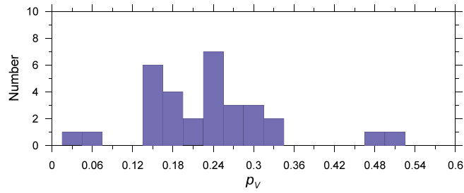
Fig. B.1. Geometric albedos p_V of asteroid pairs.
