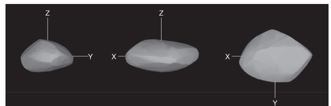
Fig. 12. Convex shape model of (25884) Asai for the pole solution (L_1, B_1) = (159^\circ, -57^\circ) .
