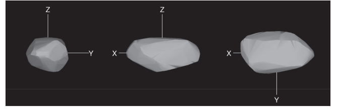
Fig. 24. Convex shape model of (60744) 2000 GB93 for the pole solution (L_1, B_1) = (202^\circ, -69^\circ) .
