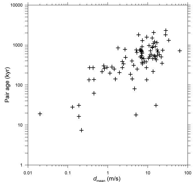
Fig. 1. Nominal estimated pair age ( T_{\text{sep}} ) vs distance of pair members in the space of mean orbital elements ( d_{\text{mean}} ) data for 89 asteroid pairs show a correlation between the two quantities. The two outlying lowermost points in the right half of the plot are young asteroid pairs with d_{\text{mean}} increased due to their irregular dynamics (see text).
