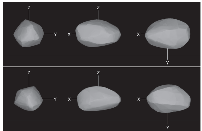
Fig. 9. Convex shape models of (5026) Martes for the pole solutions (L_1, B_1) = (11^\circ, +62^\circ) (upper panel) and (197^\circ, +47^\circ) (lower panel).
